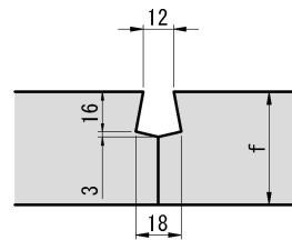
目地部詳細 2 l = 600, 1000
