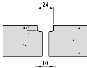
目地部詳細 1 l = 1990
