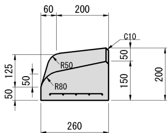
A 変形2 200/260 × 150/200 × 790
