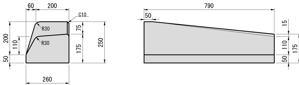
特殊 A 変形1 200/260 × 175/250 × 790 86 kg
